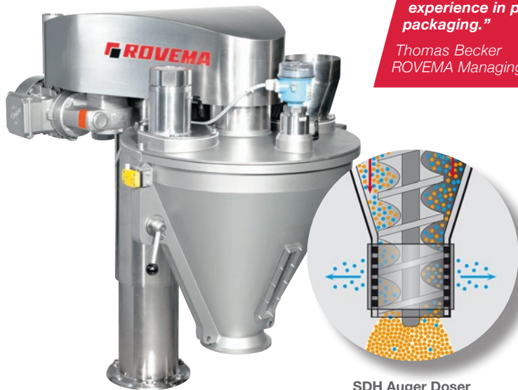
SDH Auger Doser in hygienic design
